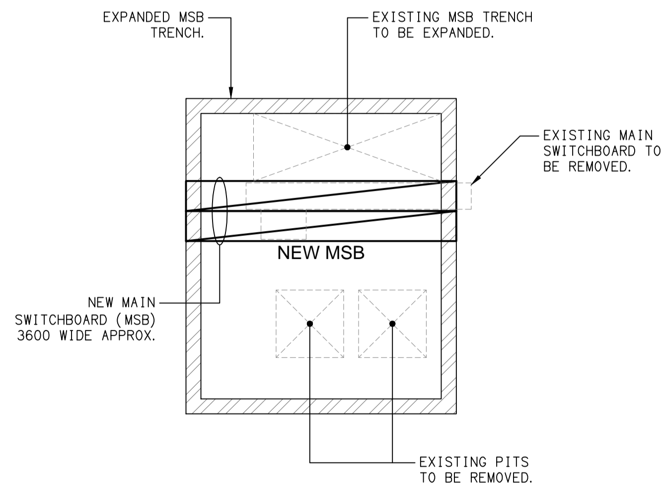
DETAIL A EXPANDED MSB TRENCH PLAN SCALE 1:50
